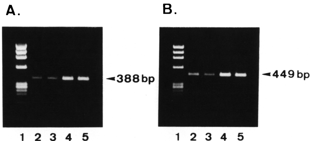
Fig. 2. Representative ethidium bromide-stained agarose gels (1.5%) of PCR products with specific primers for ACE (panel A) and mast cell chymase (panel B). Lane 1 contains \phi 174- Hae III digested DNA marker. Lanes 2 and 3 contain PCR products using RNA samples isolated from non-injured common carotid arteries. Lanes 4 and 5 contain PCR products from injured common carotid arteries. The arrowheads at 388 bp and 449 bp indicate the positions of PCR products for the ACE and mast cell chymase, respectively.
